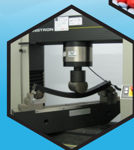
Material Testing
